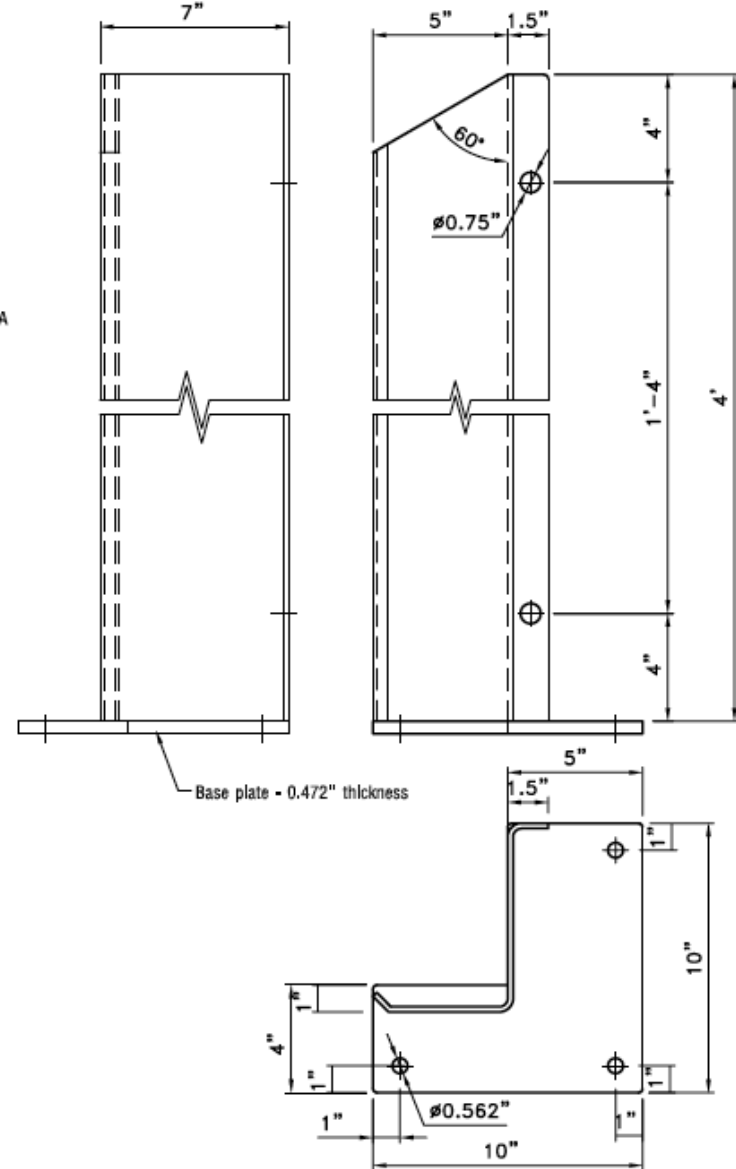
OVERHEAD DOOR TRACK GUARD 5"x7" - 48" RIGHT
