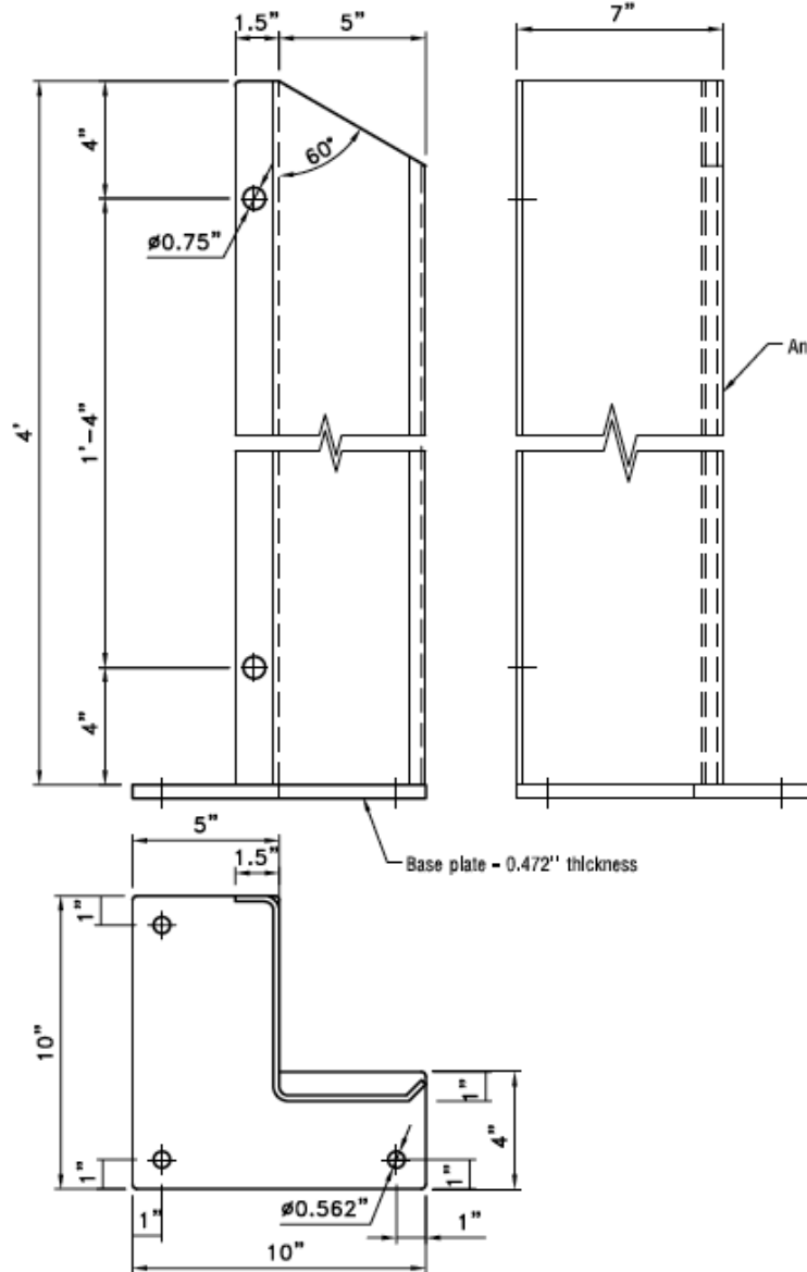
OVERHEAD DOOR TRACK GUARD 5"x7" - 48" LEFT
