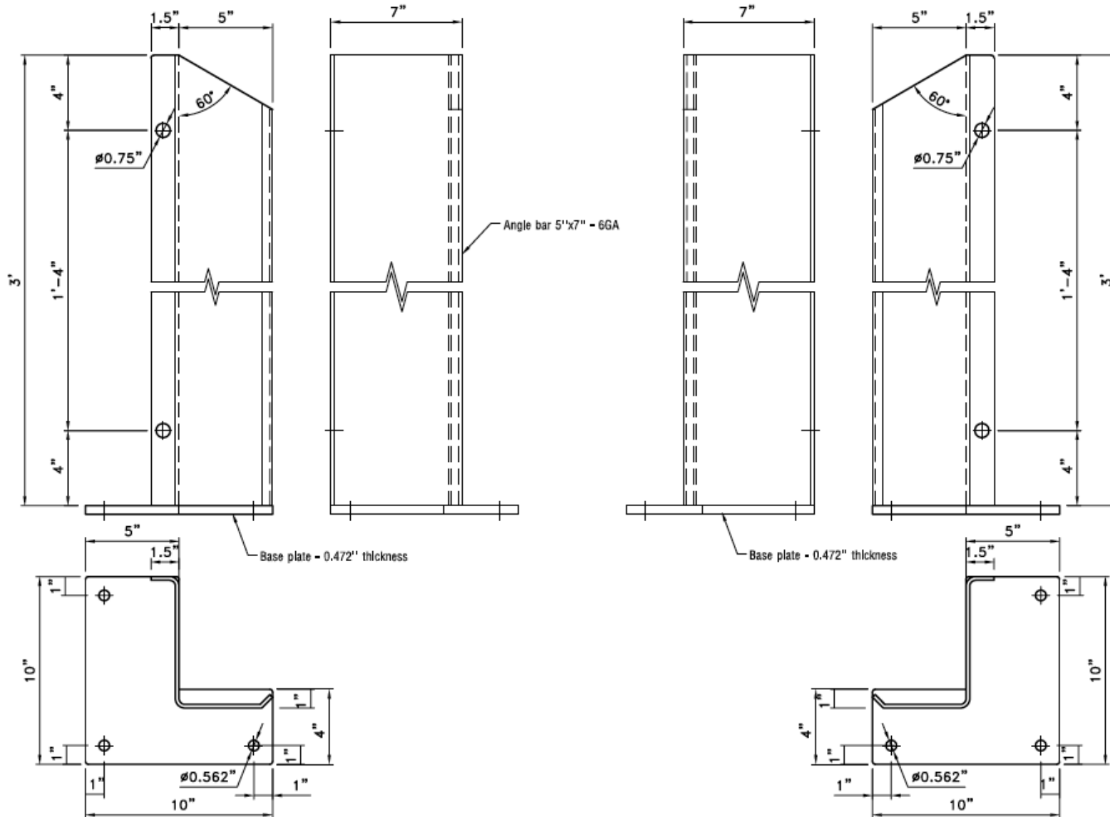
OVERHEAD DOOR TRACK GUARD 5"x7" - 36" LEFT
