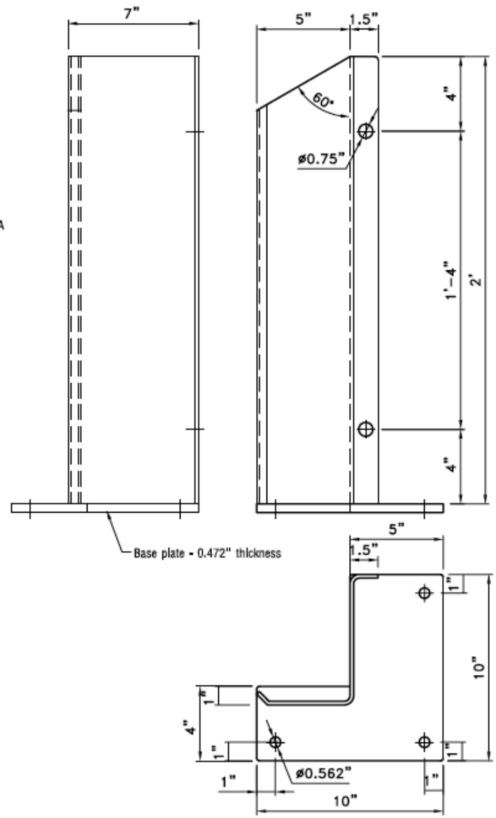
OVERHEAD DOOR TRACK GUARD 5"x7" - 24" RIGHT
