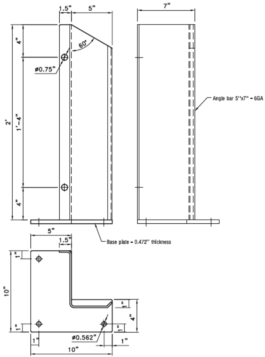
OVERHEAD DOOR TRACK GUARD 5"x7" - 24" LEFT
